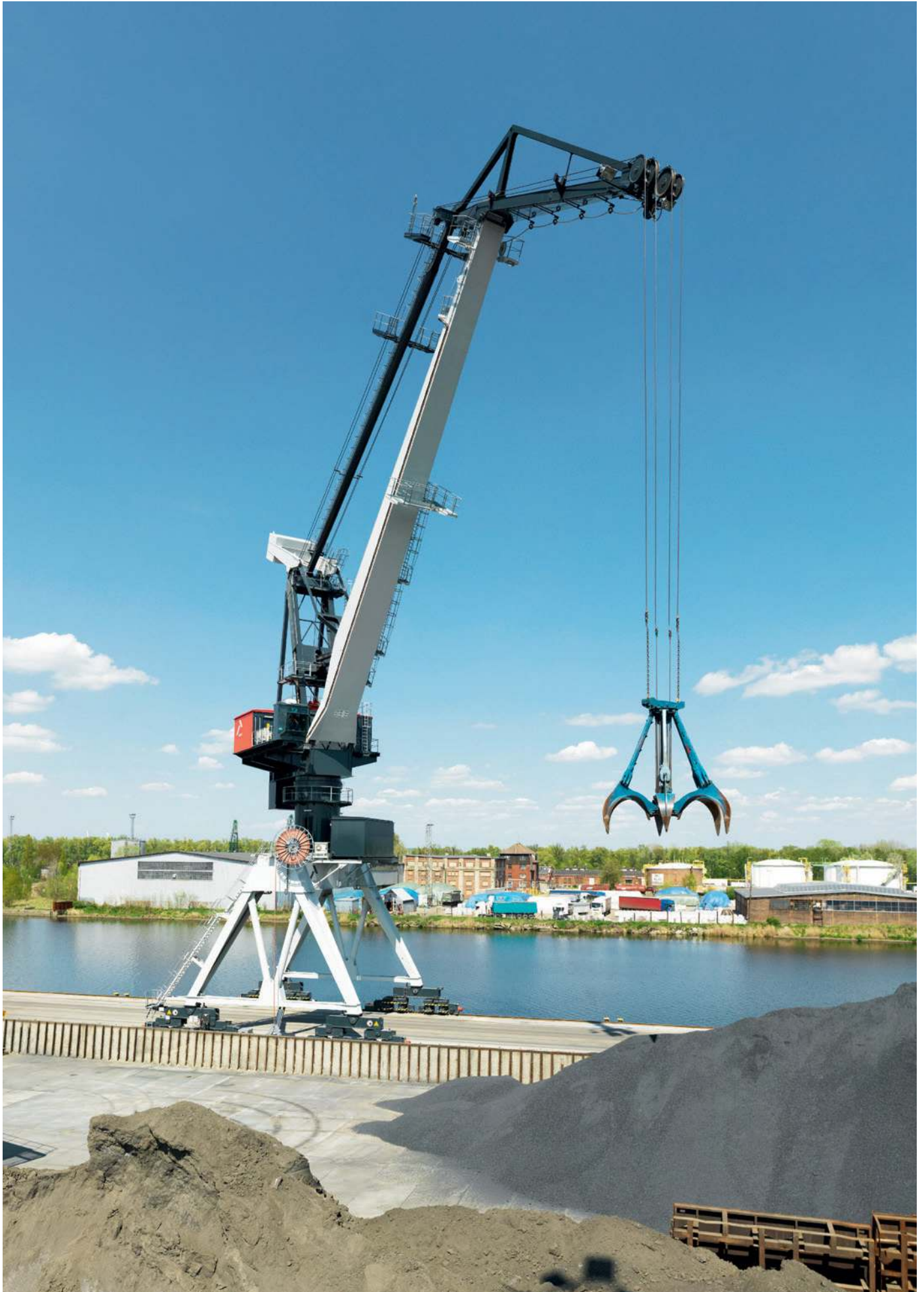
↑ From bulk goods to scrap – the Tukan M load take-up can be changed in a matter of seconds
